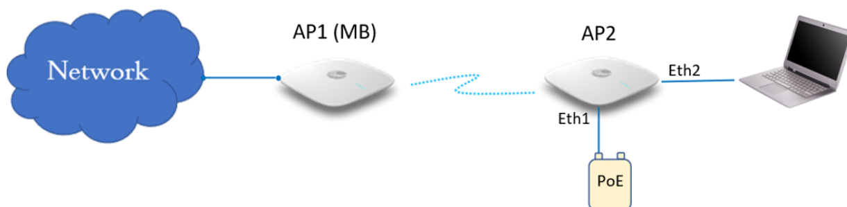
Figure 75: Deployment Scenario 1
