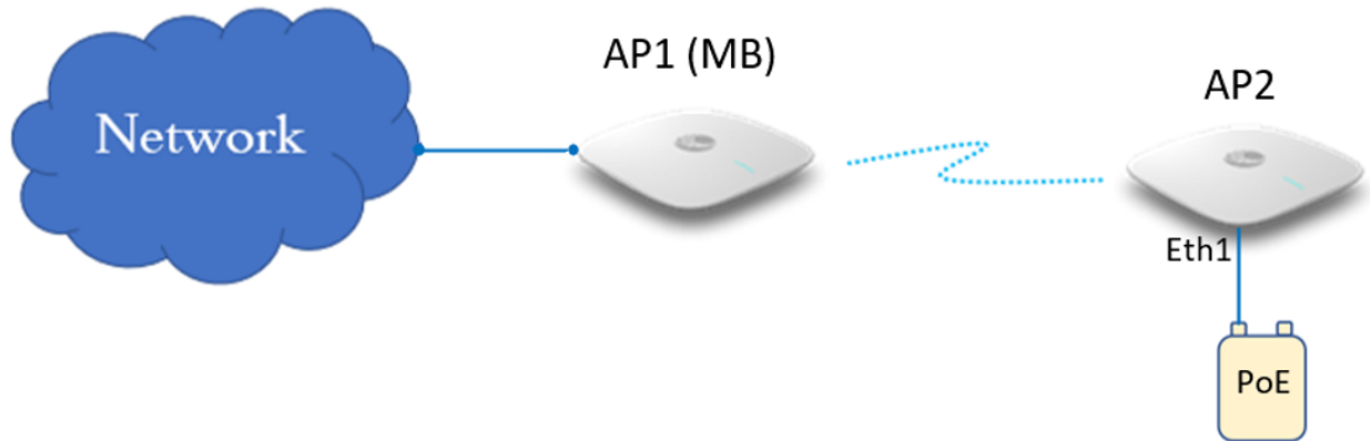
Figure 77: Deployment Scenario 3
