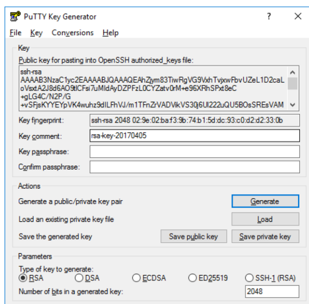
Figure 67: Public and Private Key
