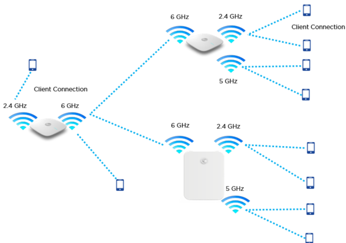
Figure 74: Single hop mesh Connection in 6 GHz with two Mesh Clients
