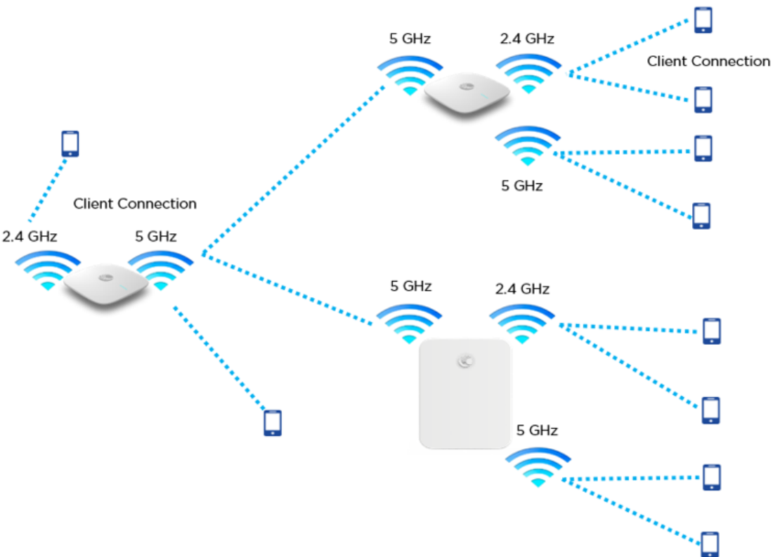
Figure 73: Single hop mesh connection in 5 GHz with two Mesh Clients and 2.4 GHz and 5 GHz as access
